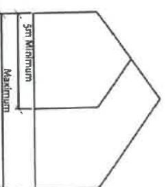
Figure 4: Building width: Core Buildings Type I erf.
