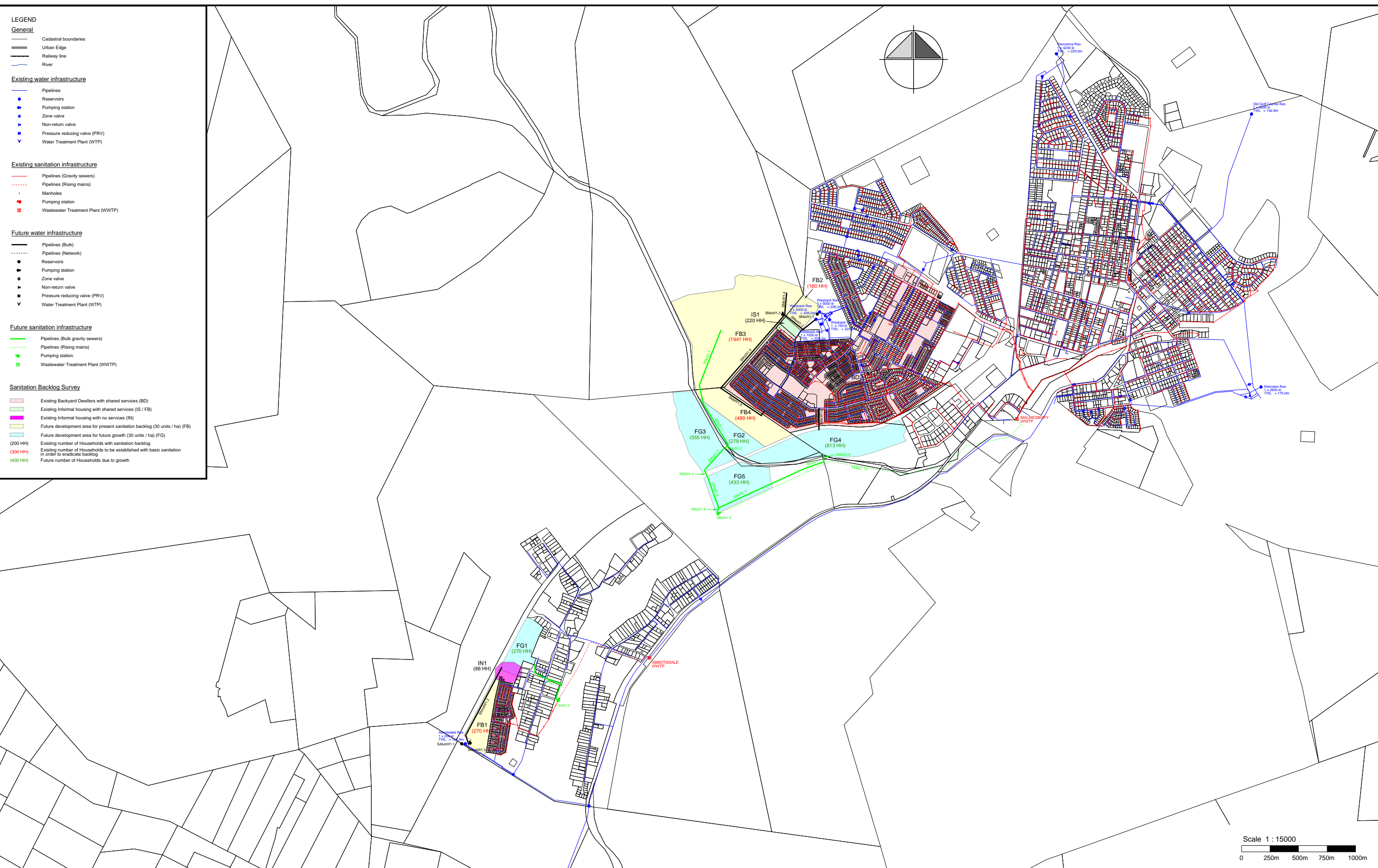
Figure 2401 Swartland:- Abbotsdale / Malmesbury Survey results and required bulk works for water and sanitation
